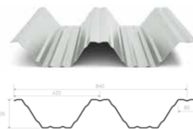
Trapezblech S135/420
