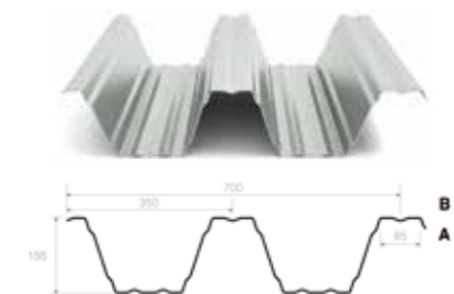
Trapezblech S158/350
