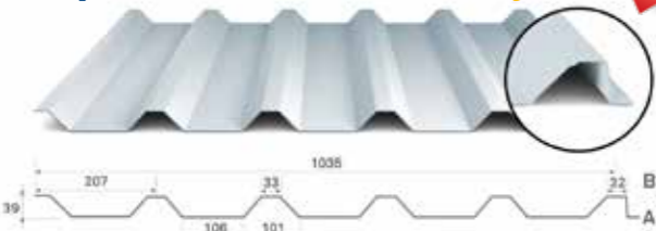
Trapezblech S35/207.PLUS easy FIX
