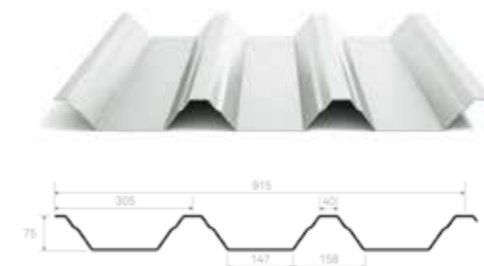
Trapezblech S75/305
